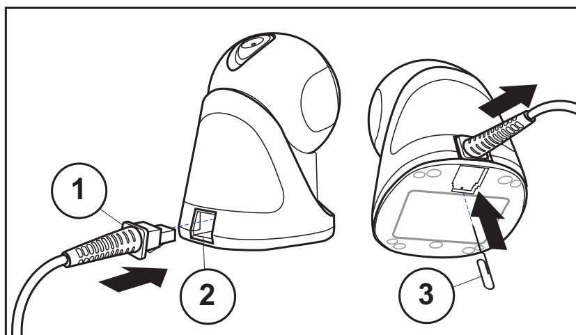
Figure 1. Cable Connection/Disconnection at the Scanner
